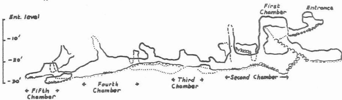
Projected Section on 127°
